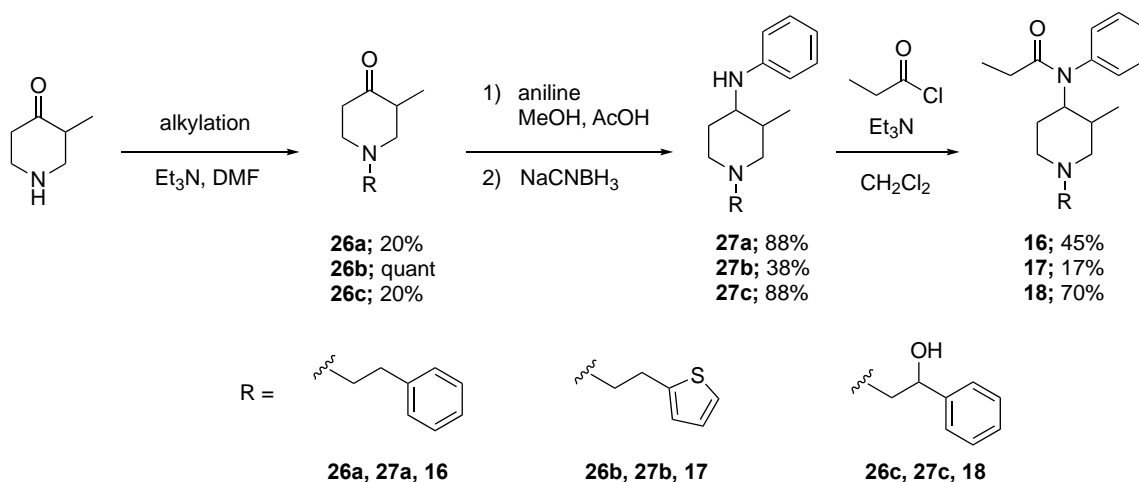
Scheme 4. The synthesis of 3-methyl derivatives 16–18
