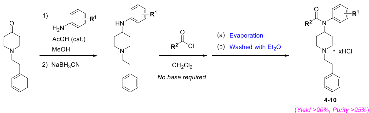
Scheme 2. Preparation of fentanyl hydrochloride by modified Siegfried method (Current study)
