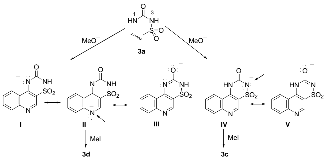
Scheme 6
