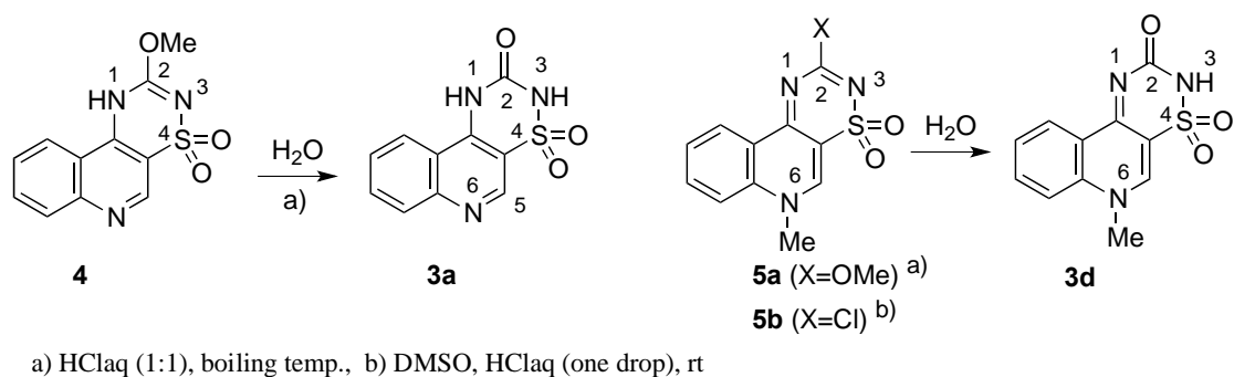
Scheme 3
