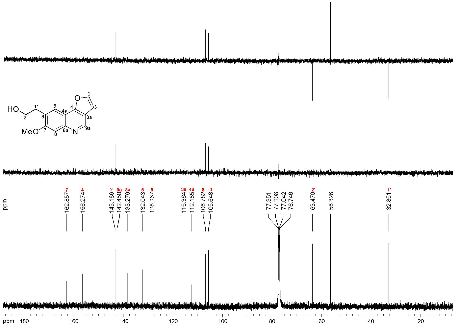
Figure S5 ^{13}\text{C} NMR spectrum of 2-(7-methoxyfuro[3,2- c ]quinolin-6-yl)ethanol (2)
