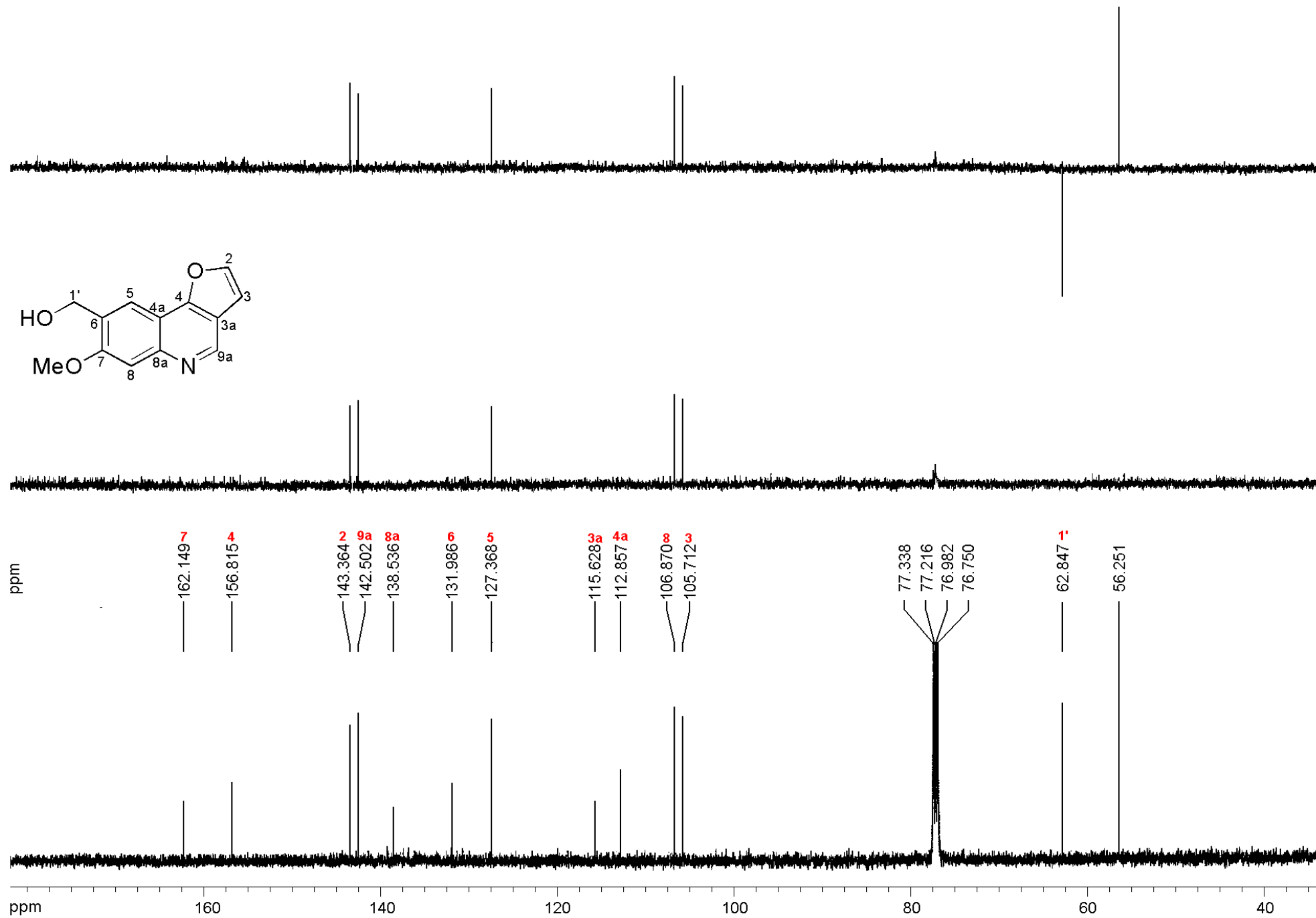
Figure S9 13 C NMR spectrum of (7-methoxyfuro[3,2- c ]quinolin-6-yl)methanol ( 3 )
