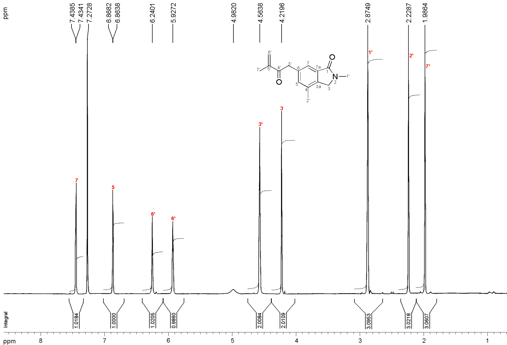
Figure S11. 1 H NMR spectrum of 1 , the compound had been purified again.
