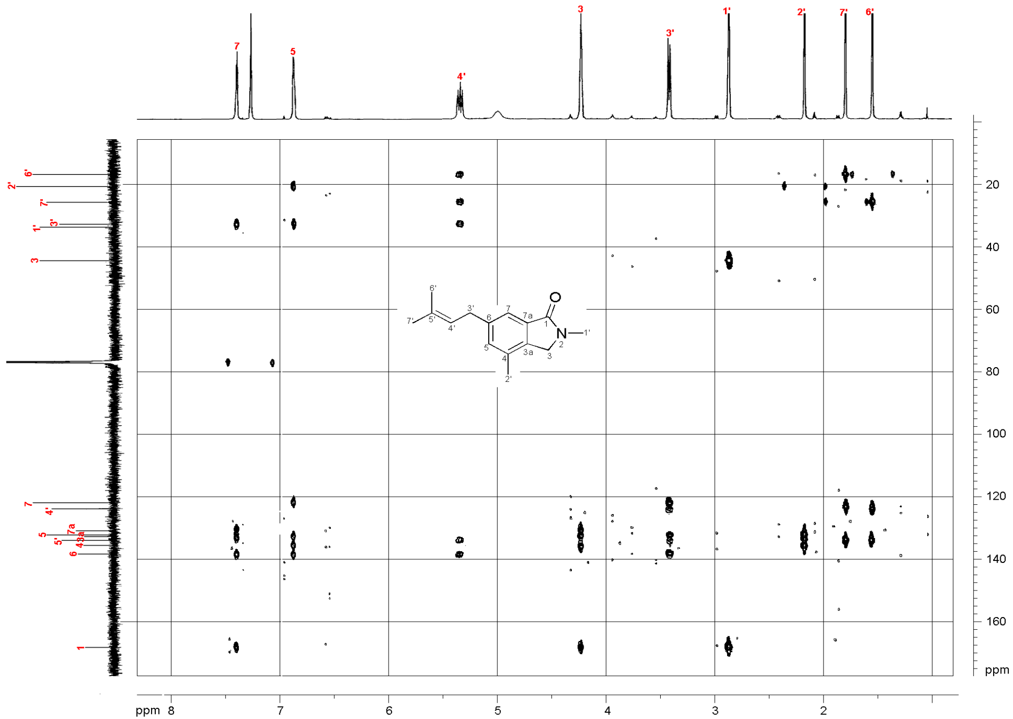
Figure S10. HMBC NMR spectrum of 2,4-dimethyl-6-(3-methylbut-2-enyl)isoindolin-1-one (3)
