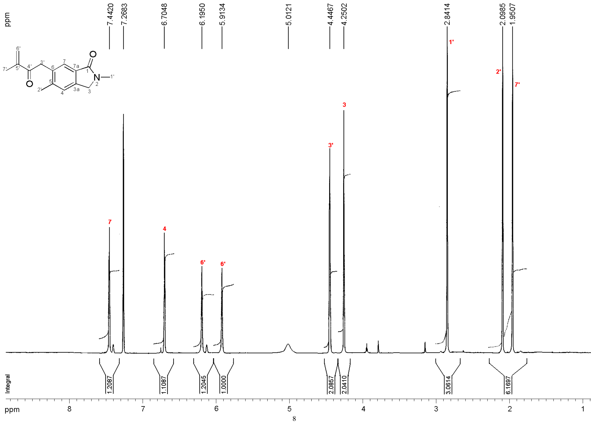
Figure S6. 1 H NMR spectrum of 2,5-dimethyl-6-(3-methyl-2-oxobut-3-enyl)isoindolin-1-one (2)
