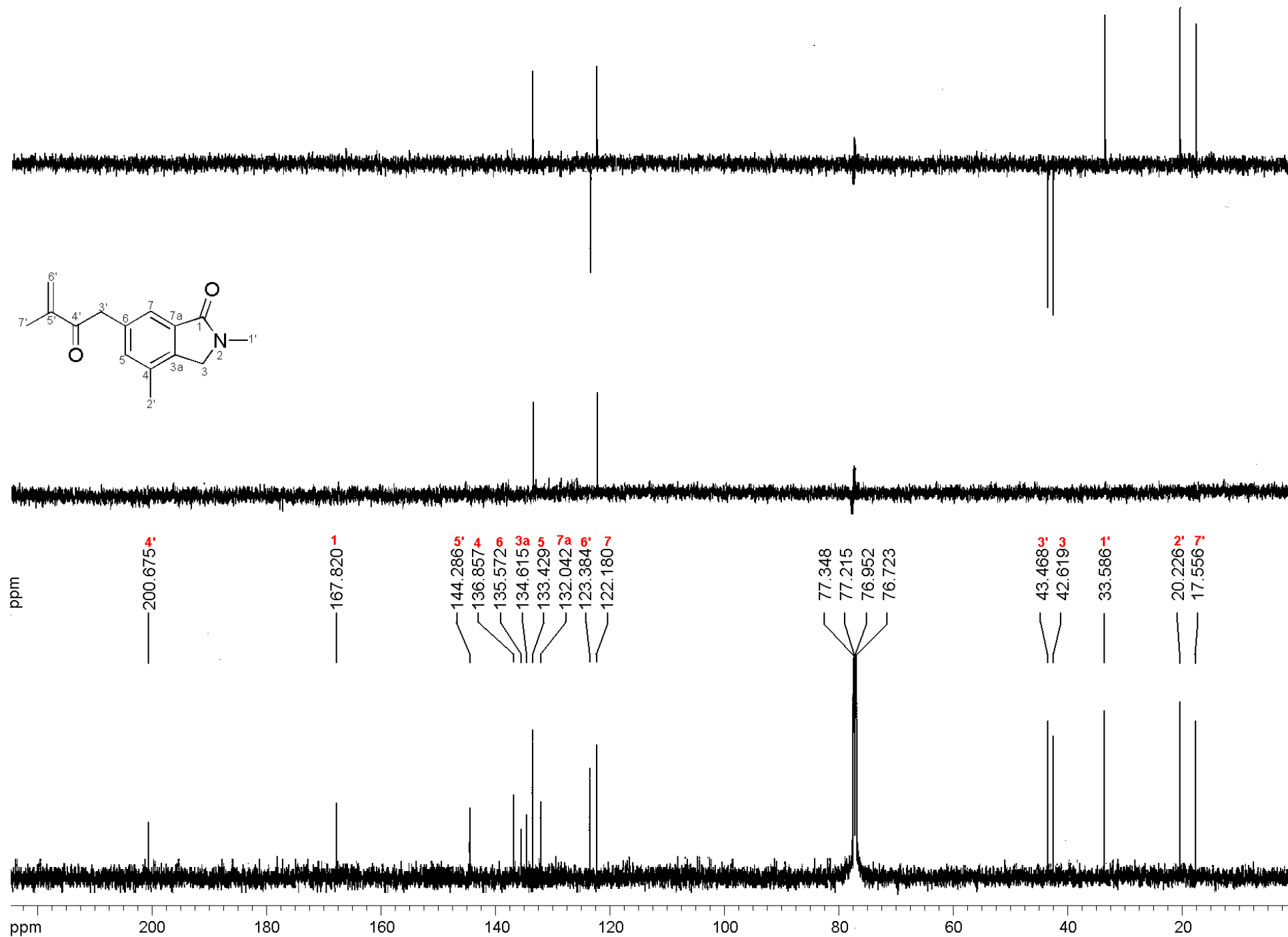
Figure S1. ^{13}\text{C} and DEPT NMR spectra of 2,4-dimethyl-6-(3-methyl-2-oxobut-3-enyl)isoindolin-1-one ( 1 )
