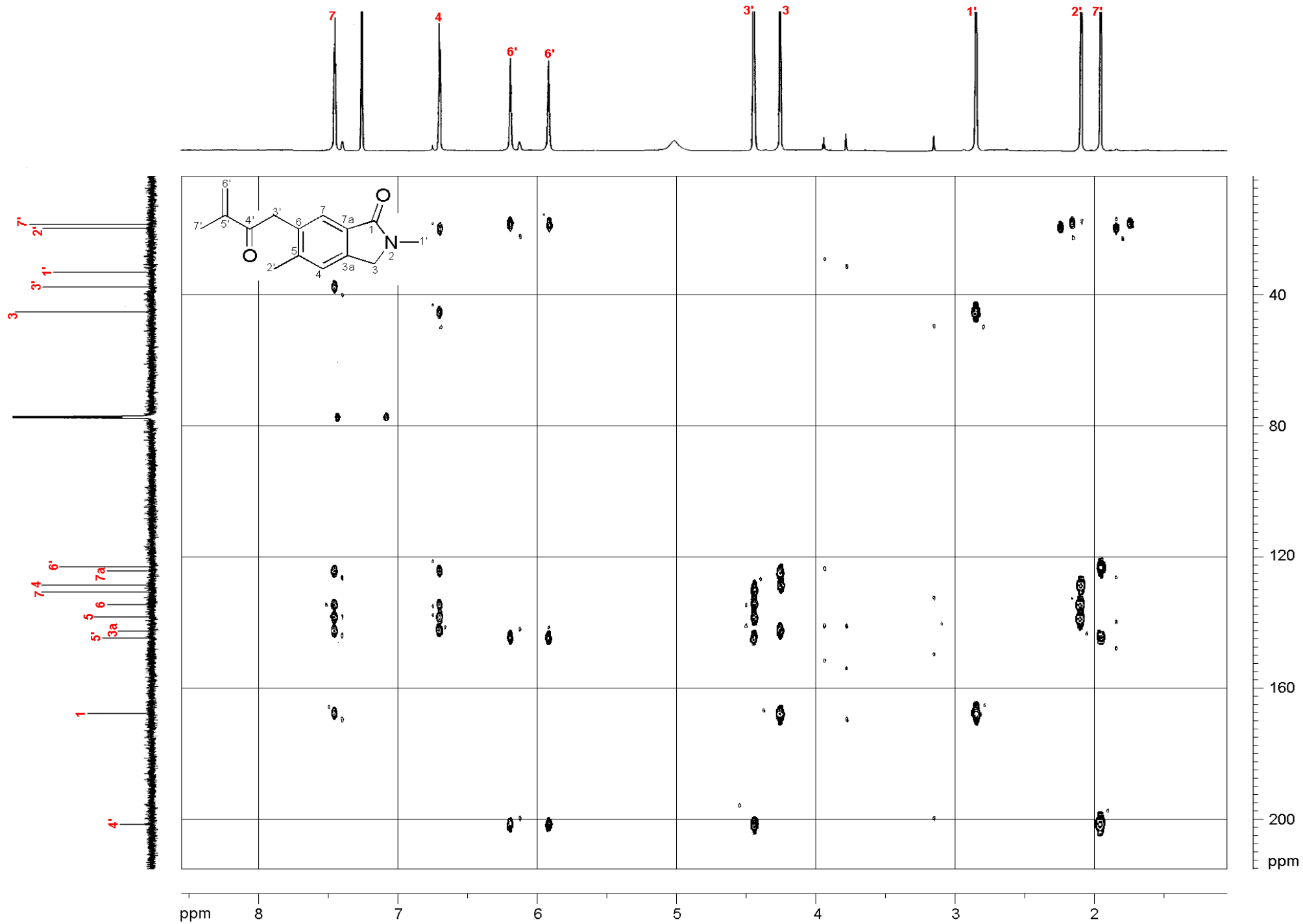
Figure S7. HMBC NMR spectrum of 2,5-dimethyl-6-(3-methyl-2-oxobut-3-enyl)isoindolin-1-one (2)
