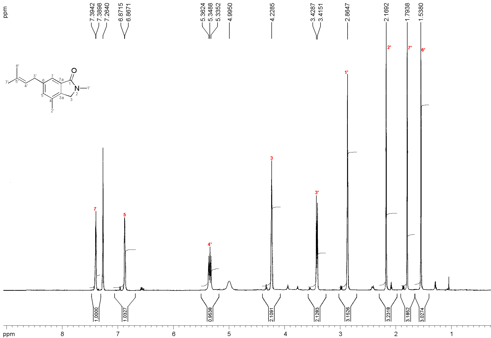
Figure S9. ^1\text{H} NMR spectrum of 2,4-dimethyl-6-(3-methylbut-2-enyl)isoindolin-1-one ( 3 )
