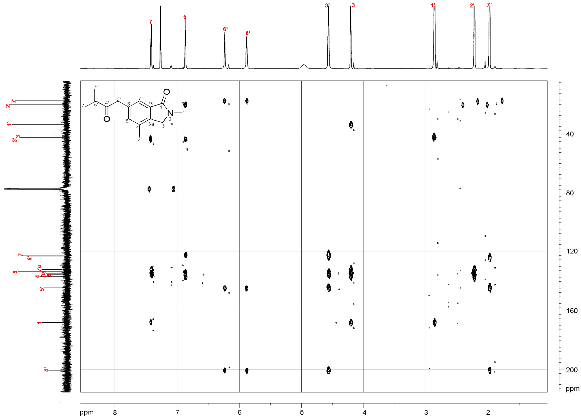
Figure S4. HMBC NMR spectrum of 2,4-dimethyl-6-(3-methyl-2-oxobut-3-enyl)isoindolin-1-one (1)
