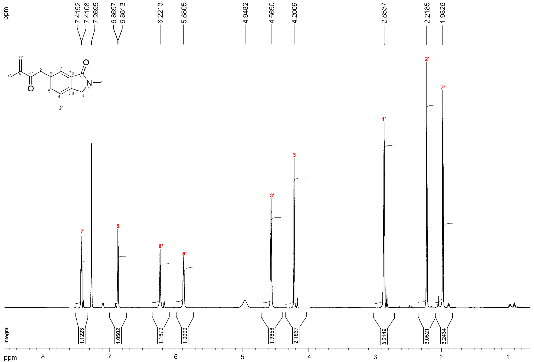
Figure S2. ^1\text{H} NMR spectrum of 2,4-dimethyl-6-(3-methyl-2-oxobut-3-enyl)isoindolin-1-one ( 1 )
