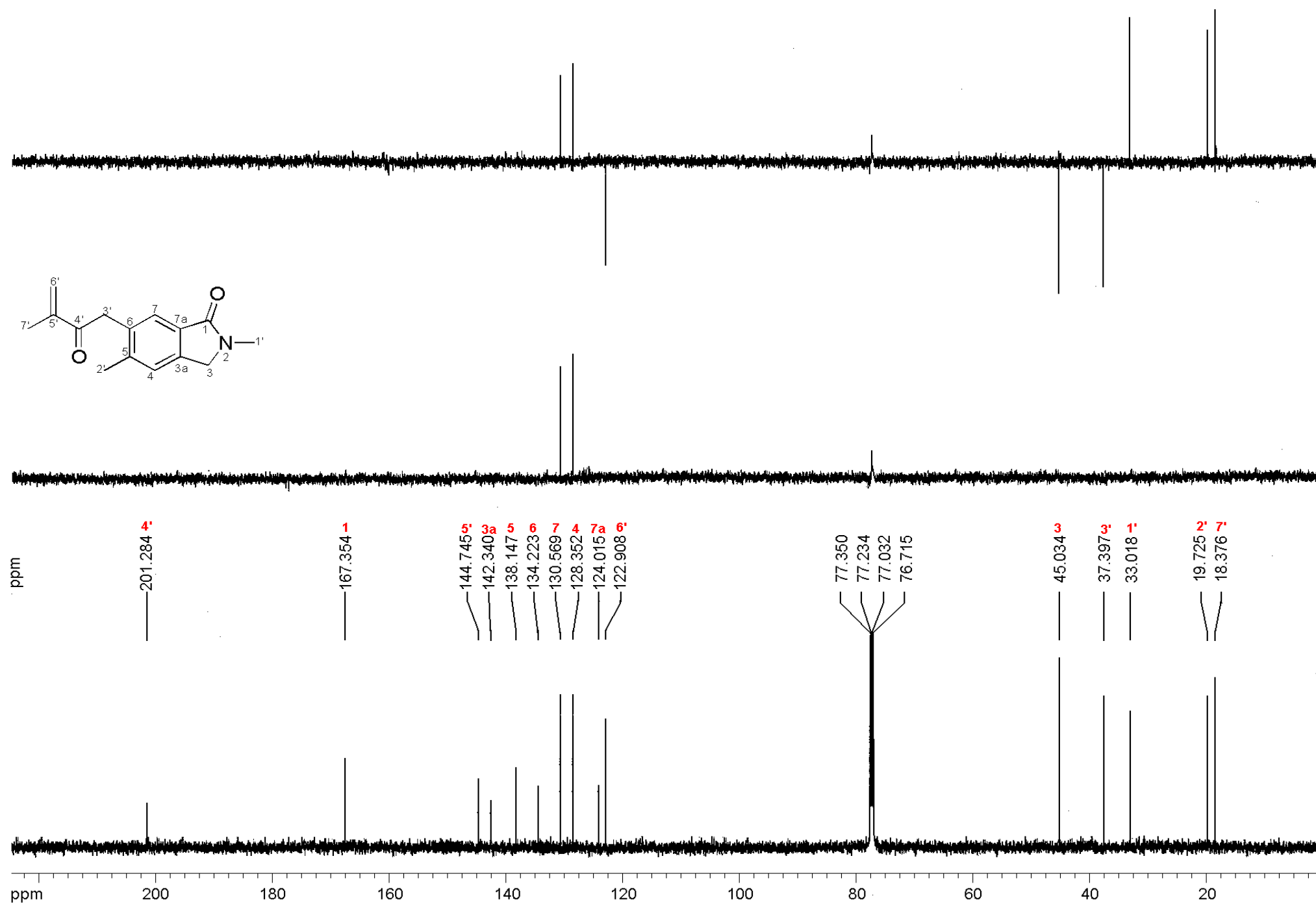
Figure S5. ^{13}\text{C} and DEPT NMR spectra of 2,5-dimethyl-6-(3-methyl-2-oxobut-3-enyl)isoindolin-1-one (2)
