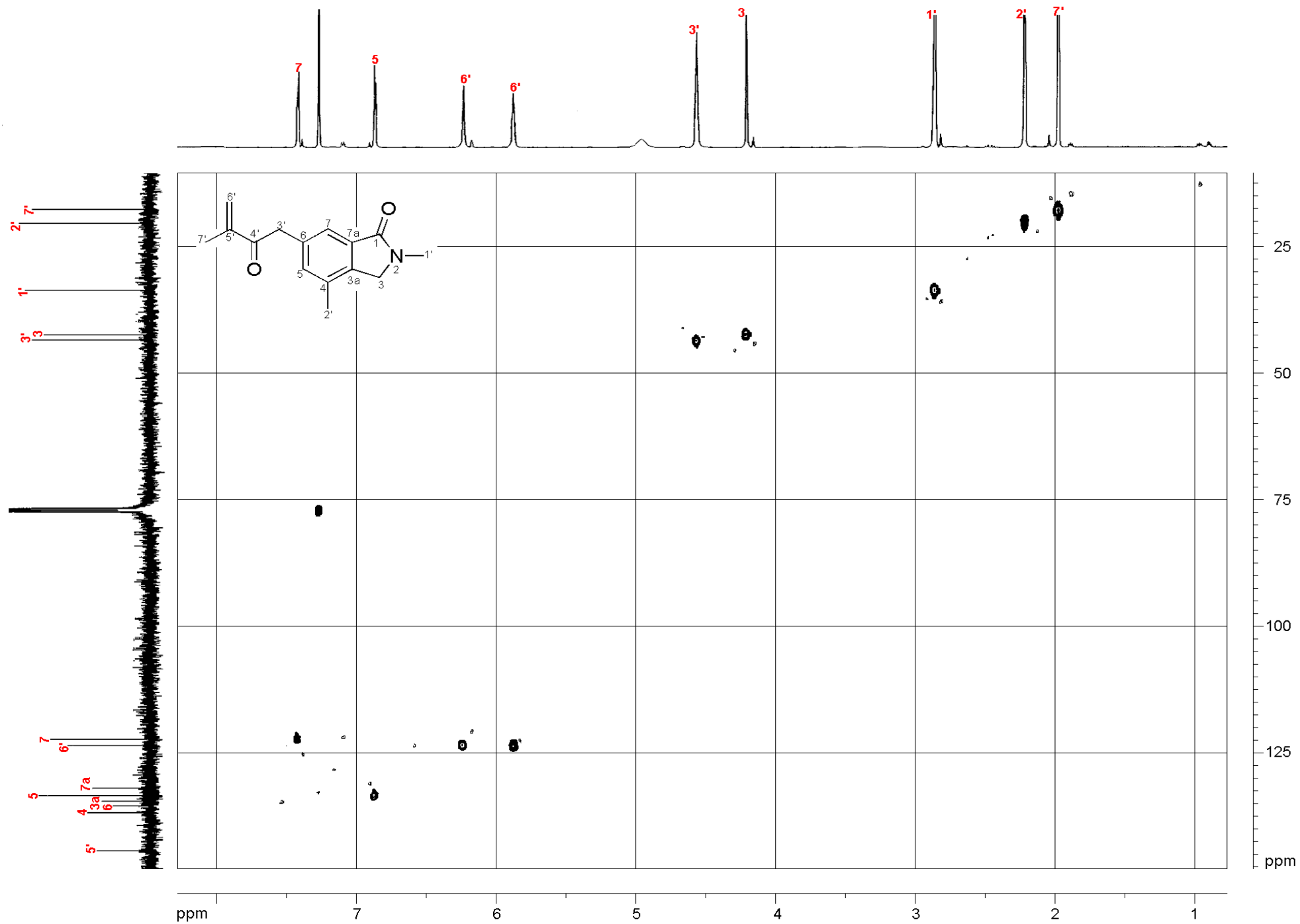
Figure S3. HSQC NMR spectrum of 2,4-dimethyl-6-(3-methyl-2-oxobut-3-enyl)isoindolin-1-one ( 1 )
