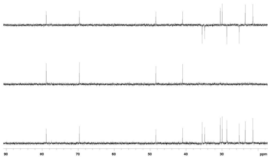
S6. DEPT spectrum of compound 1 in \text{CDCl}_3
