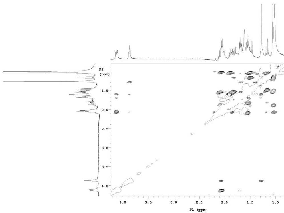
S10. NOESY spectrum of compound 1 in CDCl 3
