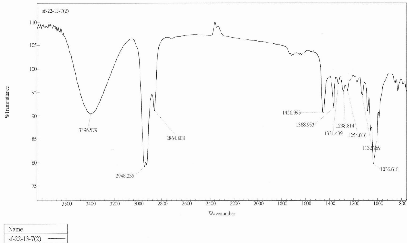
S3. IR spectrum of compound 1
