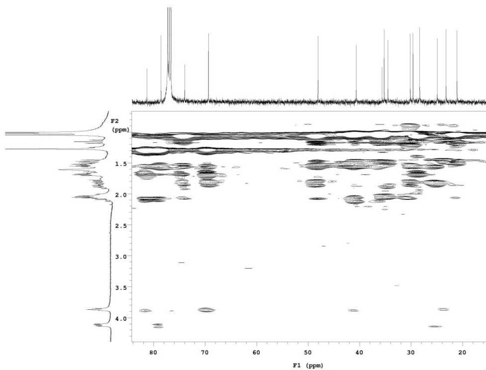
S9. HMBC spectrum of compound 1 in CDCl 3
