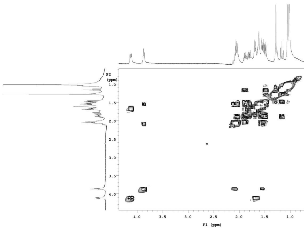
S7. ^1\text{H} - ^1\text{H} COSY spectrum of compound 1 in \text{CDCl}_3
