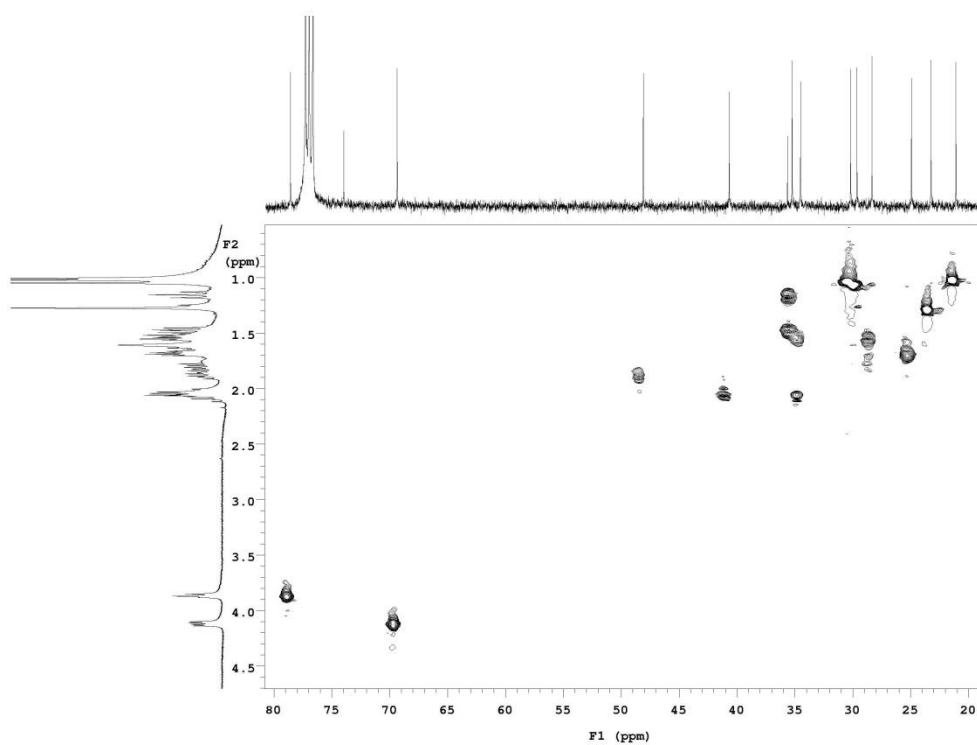
S8. HSQC spectrum of compound 1 in CDCl 3
