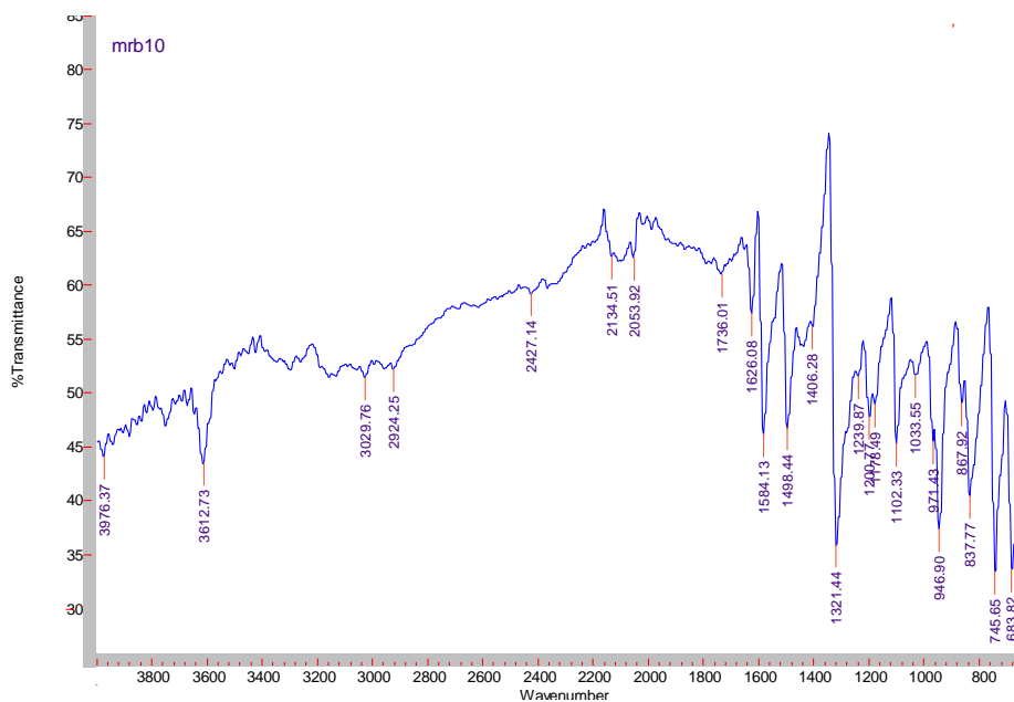
Figure S5: IR spectrum of 2b.
