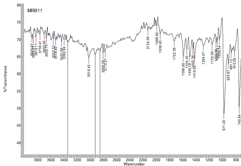
Figure S1: IR spectrum of 2a.
