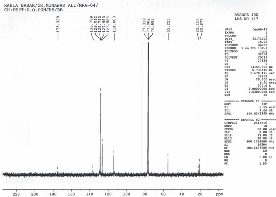
Figure S12: ^{13}\text{C} NMR spectrum of 2c.
