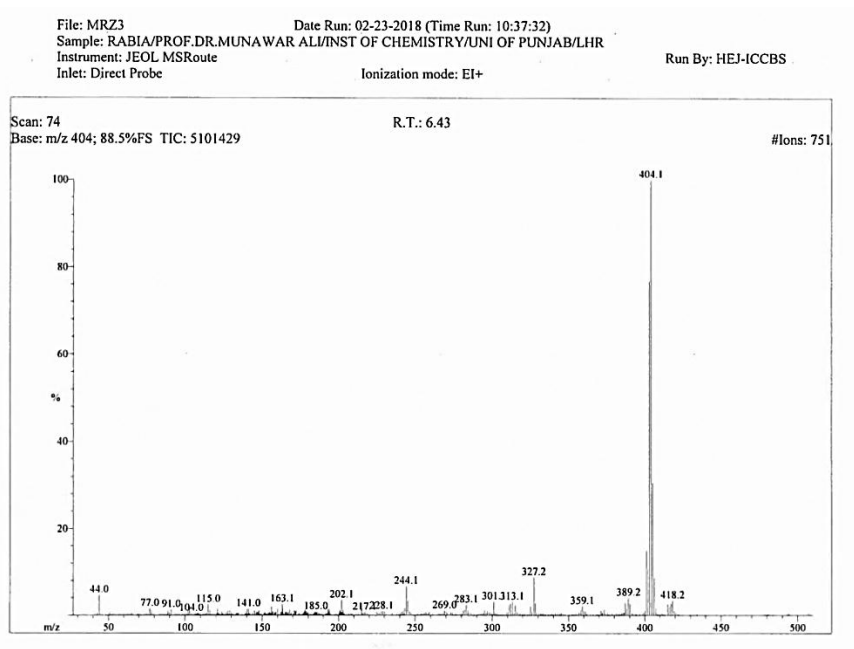
Figure S10: Mass spectrum of 2c.
