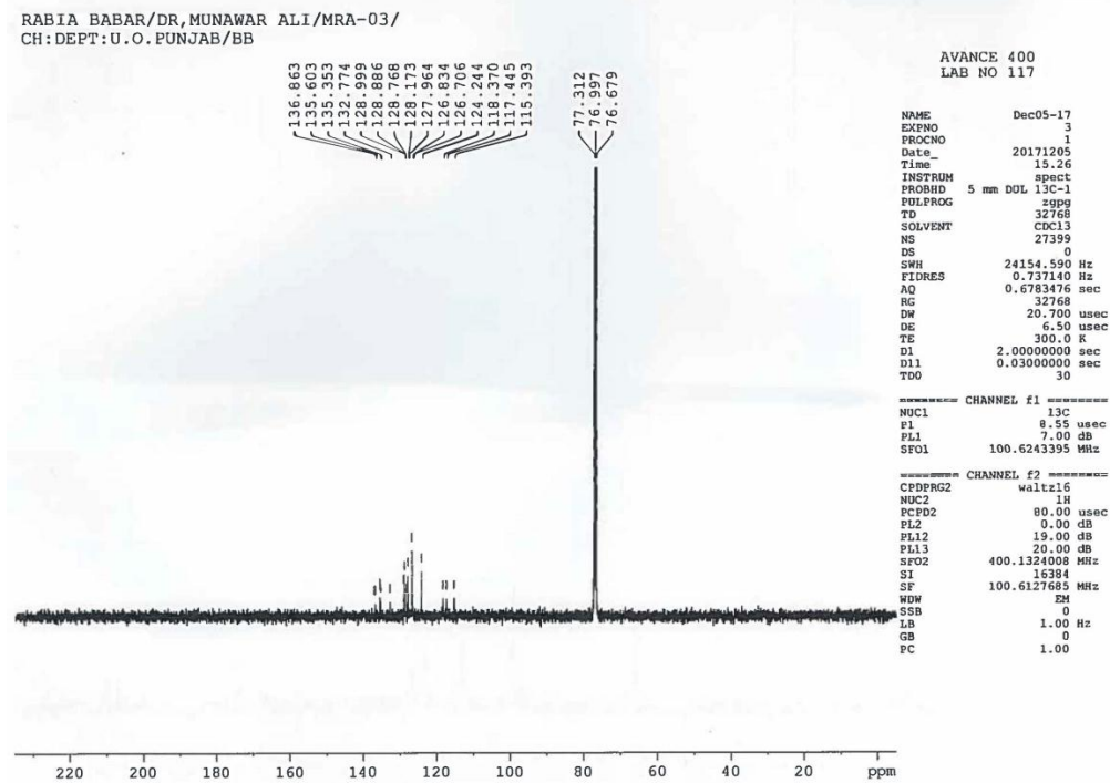
Figure S8: ^{13}\text{C} NMR spectrum of 2b
