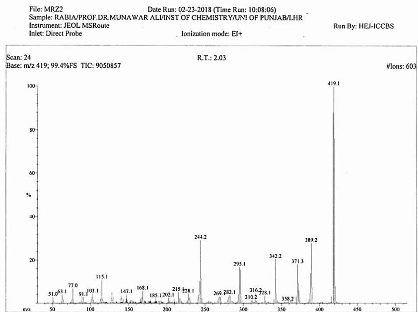
Figure S6: Mass spectrum of 2b.
