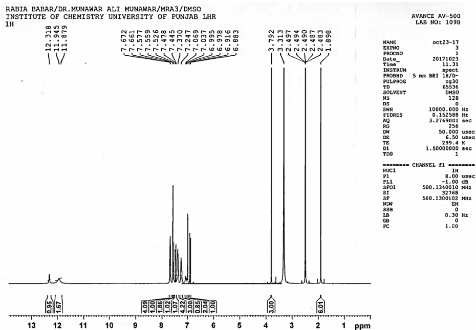
Figure S11: ^1\text{H} NMR spectrum of 2c.
