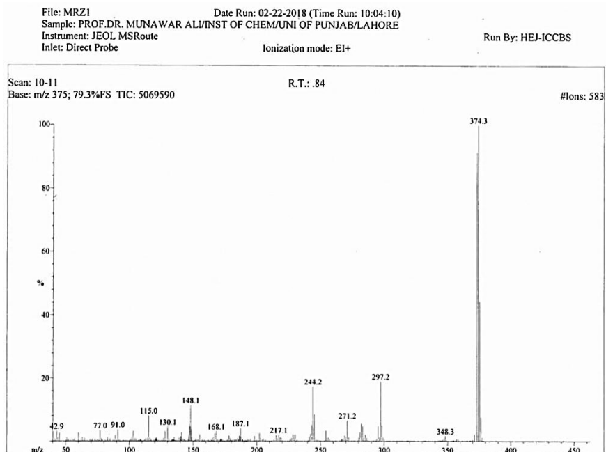
Figure S2: Mass spectrum of 2a.
