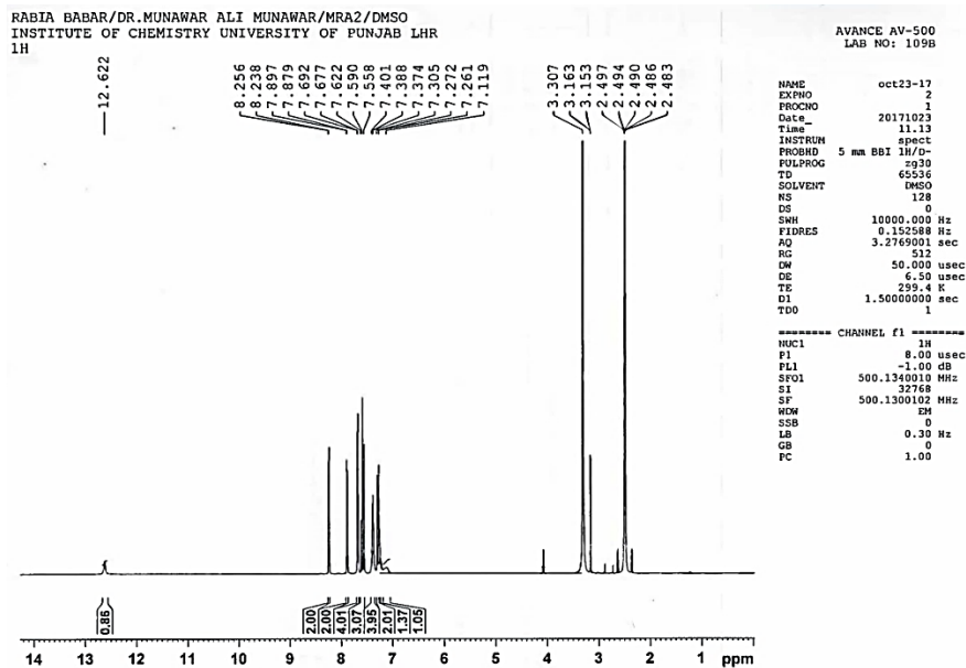
Figure S7: ^1\text{H} NMR spectrum of 2b.
