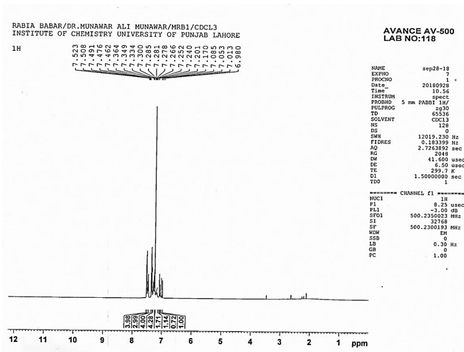
Figure S3: 1 H NMR spectrum of 2a.
