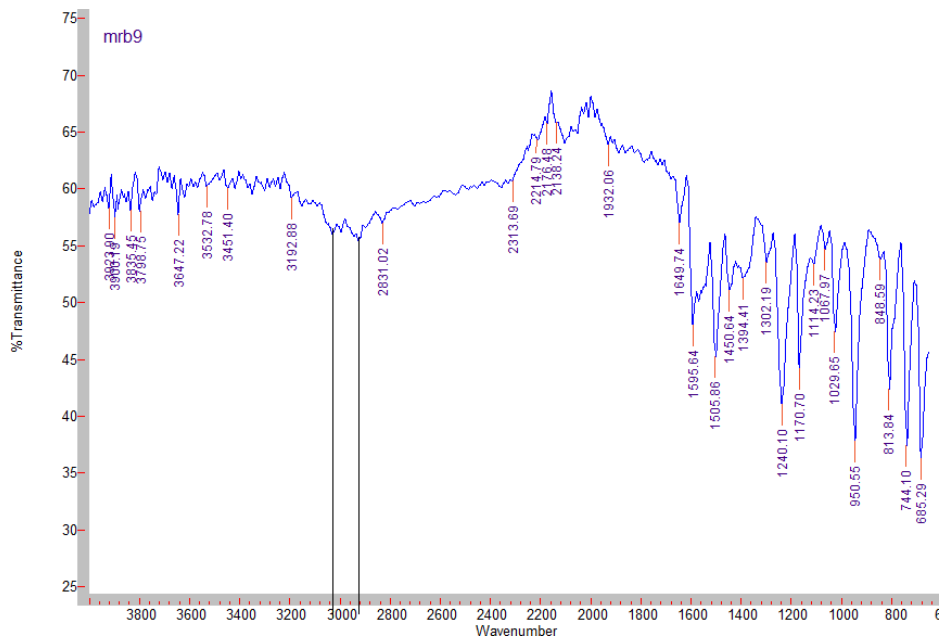
Figure S9: IR spectrum of 2c.
