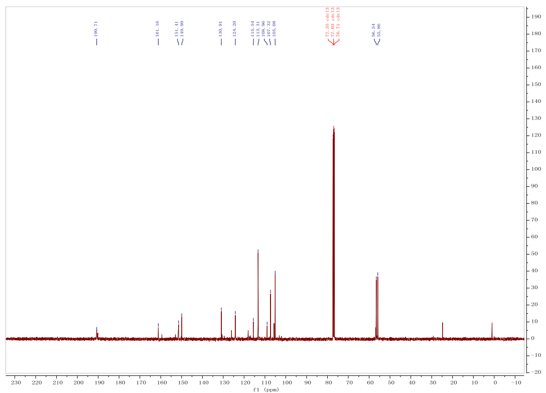
Figure 8. The ^{13}\text{C} NMR spectrum of compound 1
