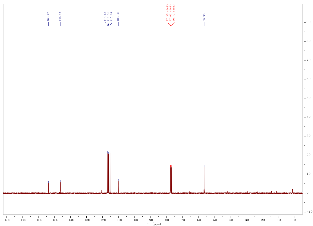
Figure 2. The ^{13}\text{C} NMR spectrum of compound 3
