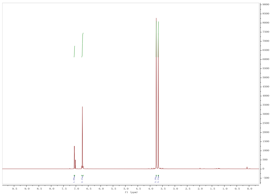
Figure 3. The ^1\text{H} NMR spectrum of compound 4
