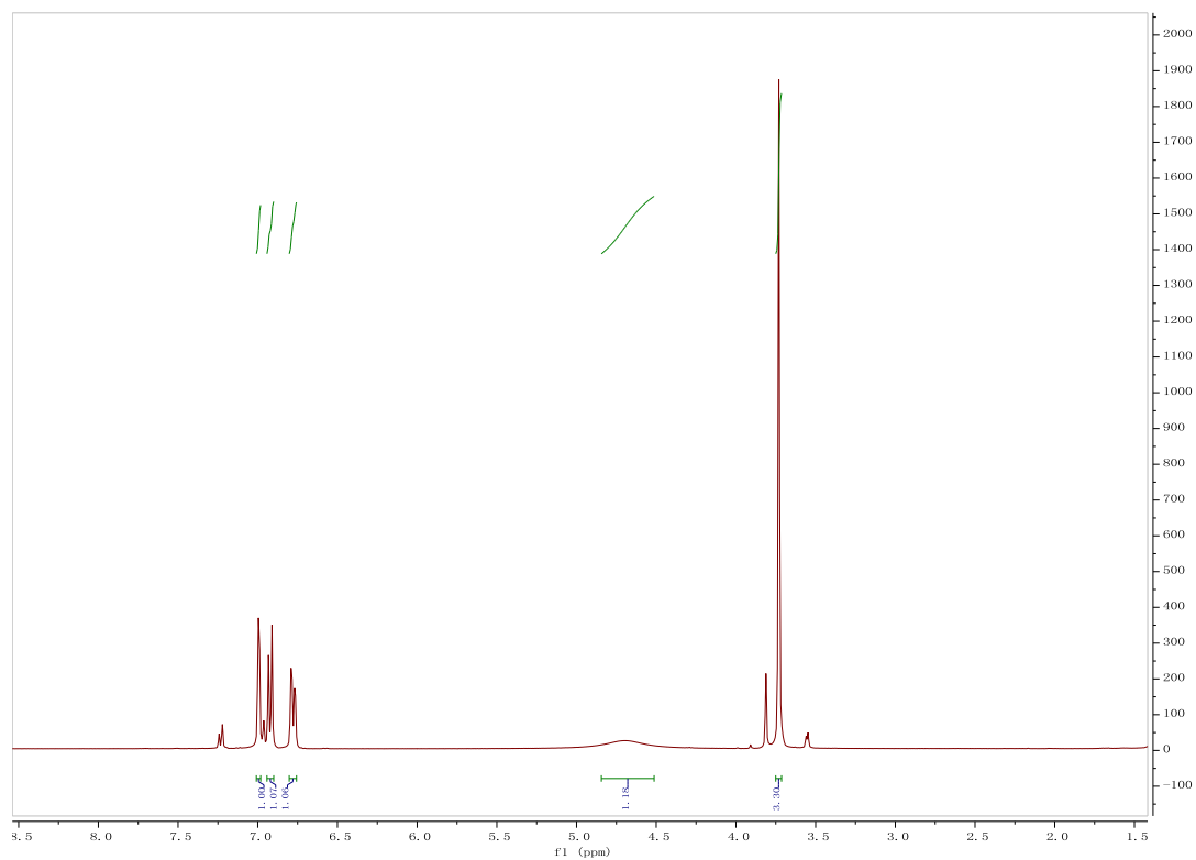
Figure 1. The ^1\text{H} NMR spectrum of compound 3
