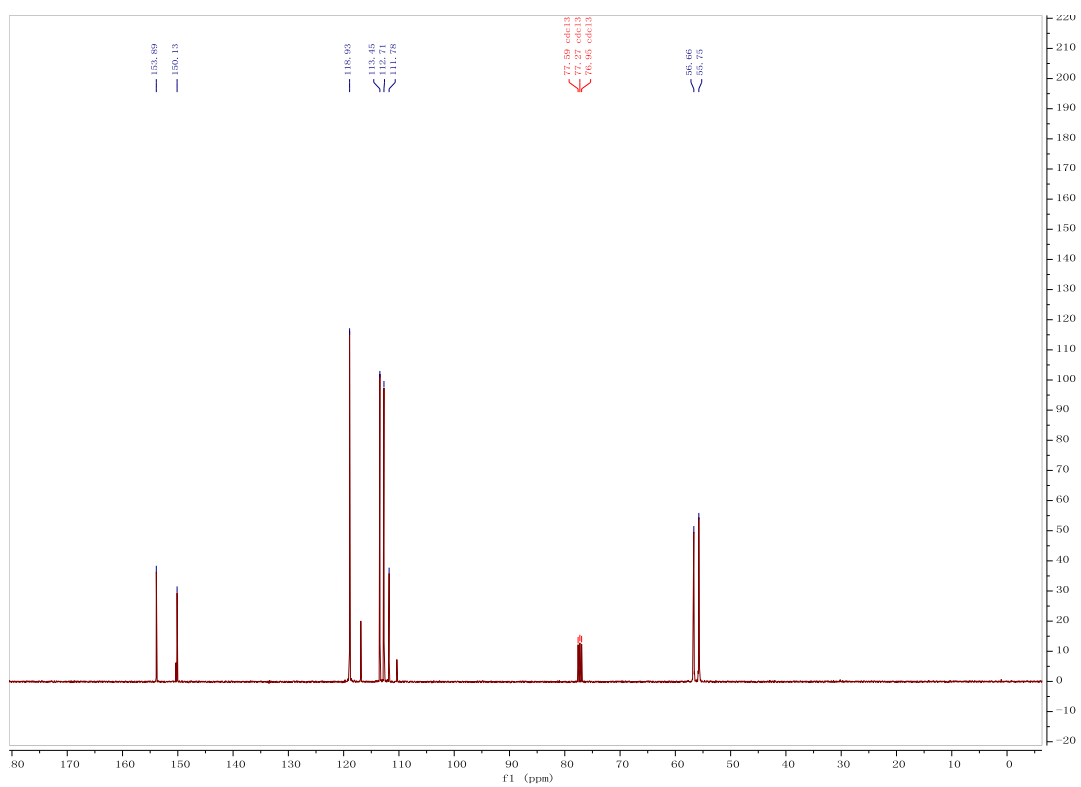
Figure 4. The ^{13}\text{C} NMR spectrum of compound 4
