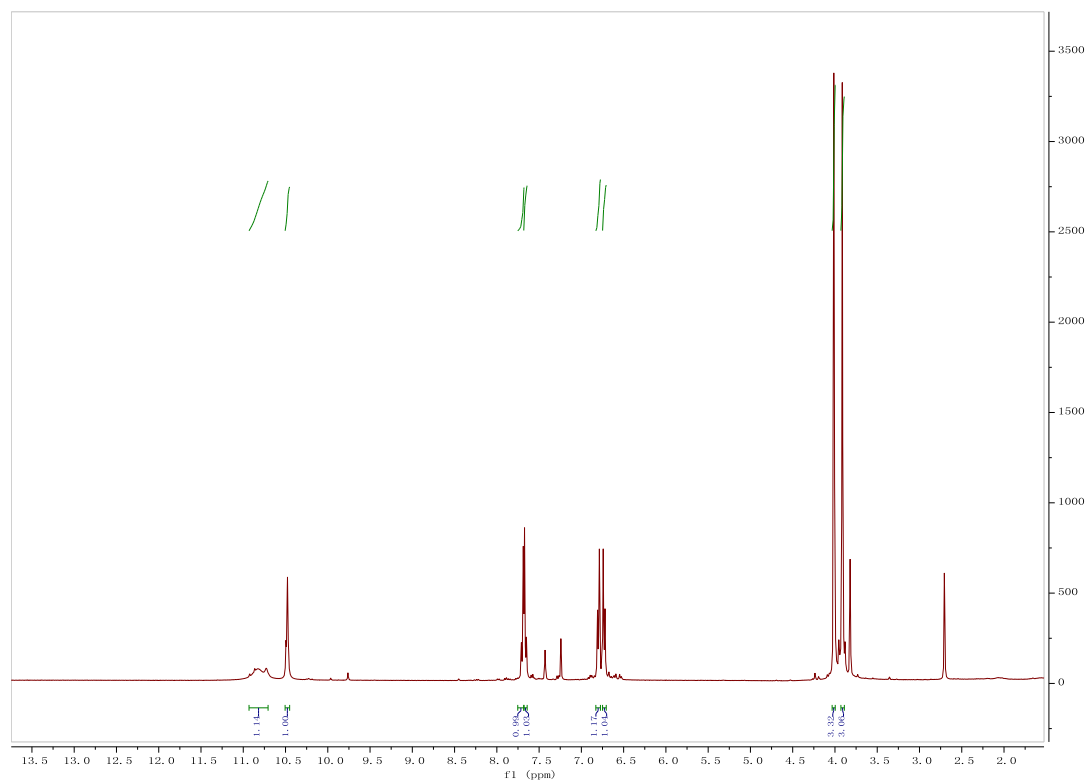
Figure 7. The ^1\text{H} NMR spectrum of compound 1
