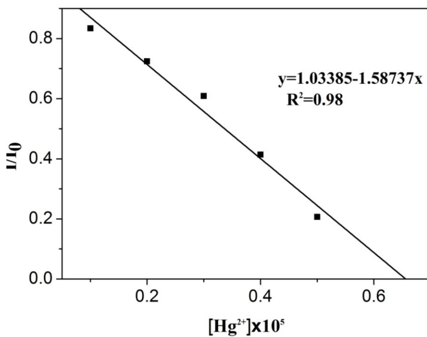
Figure S2 Stern–Volmer plots for L of weakening in presence of Hg^{2+}
