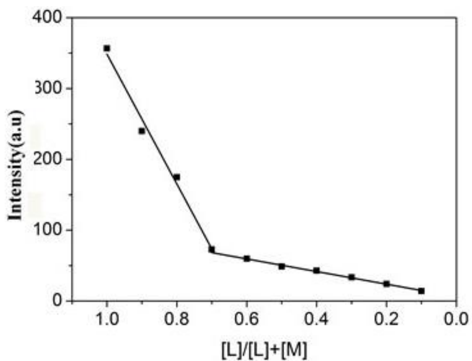
Figure S3 The Job's plot for L and \text{Hg}^{2+} ( \lambda_{\text{ex}} = 365 \text{ nm} )
