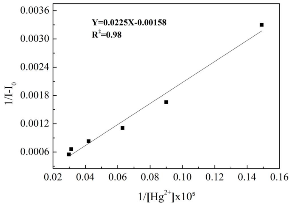
Figure S1 B-H plots for L for estimation of weakening in presence of Hg^{2+}
