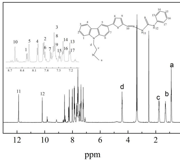
Figure S5 1 H-NMR spectrum of L
