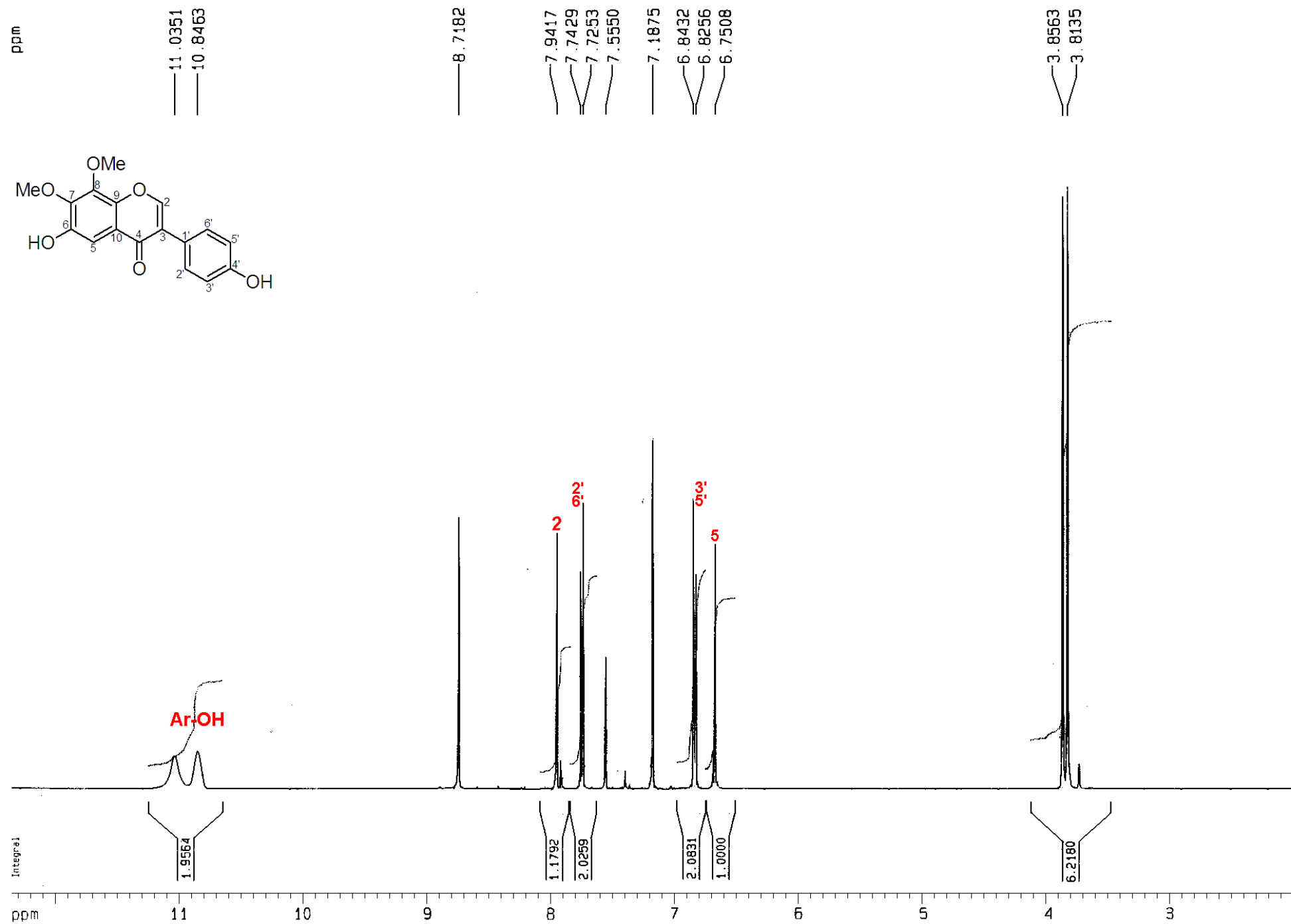
Figure S2 1 H NMR spectrum of 4',6-dihydroxy-7,8-dimethoxyisoflavone (1)
