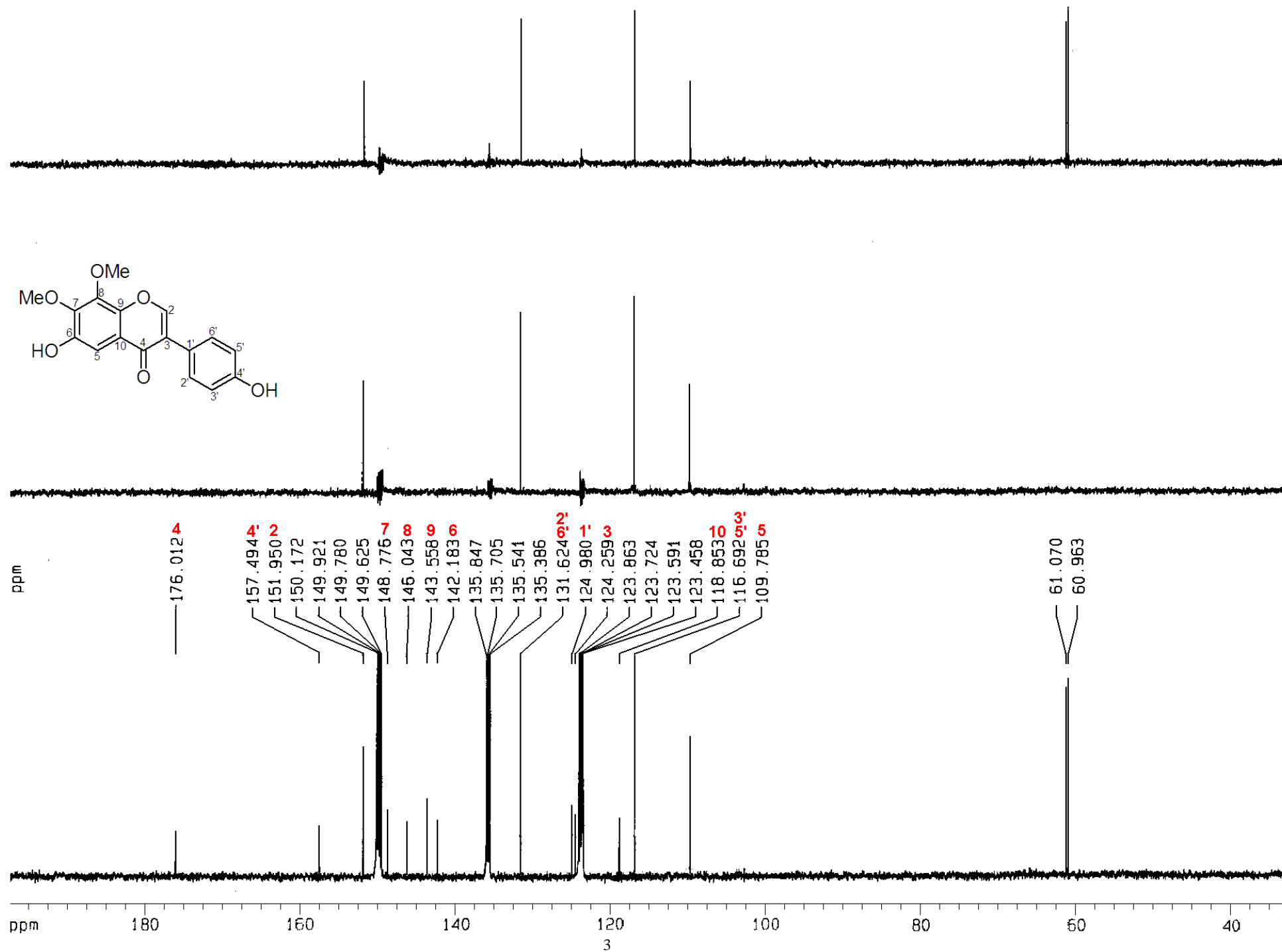
Figure S1 ^{13}\text{C} NMR spectrum of 4',6-dihydroxy-7,8-dimethoxyisoflavone ( 1 )
