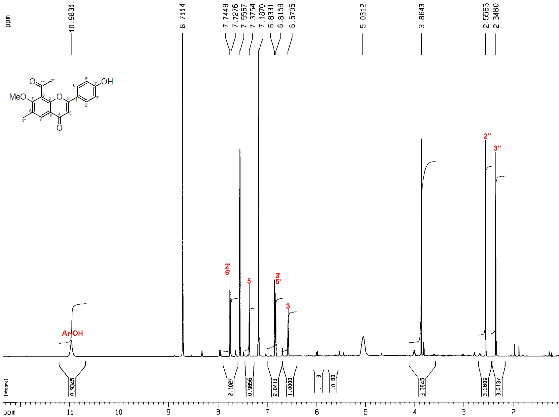
Figure S4 1 H NMR spectrum of 8-acetyl-4'-hydroxy-7-methoxy-6-methylflavone (2)
