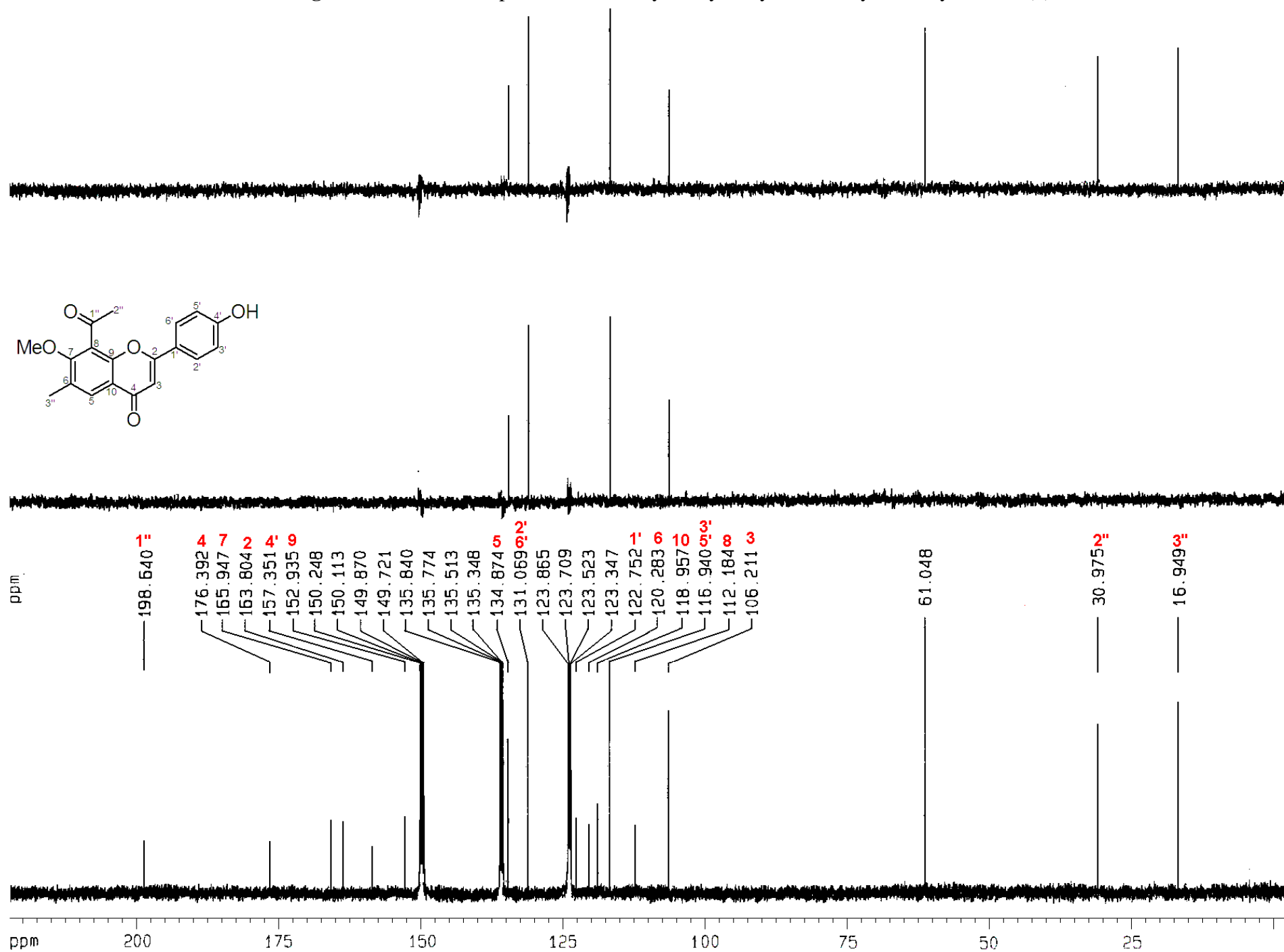
Figure S3 13 C NMR spectrum of 8-acetyl-4'-hydroxy-7-methoxy-6-methylflavone (2)
