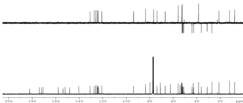
Figure 5. ^1\text{H} - ^1\text{H} COSY spectrum of 1
