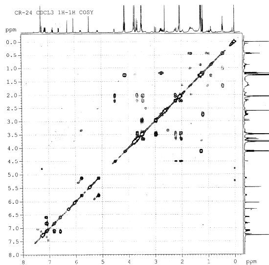
Figure 12. ^1\text{H} - ^1\text{H} COSY spectrum of 2
