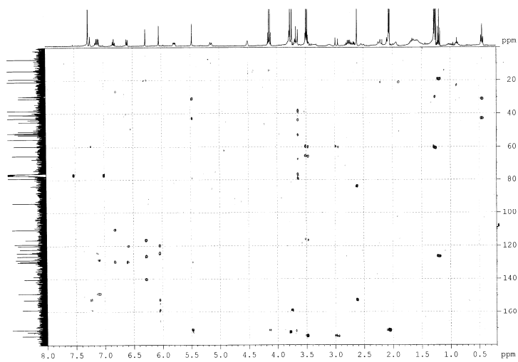
Figure 14. HMBC spectrum of 2
