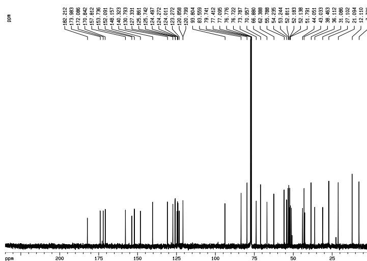
Figure 3. 13 C-NMR spectrum of 1
