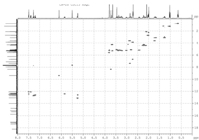
Figure 6. HSQC spectrum of 1
