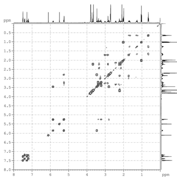
Figure 5. ^1\text{H} - ^1\text{H} COSY spectrum of 1
