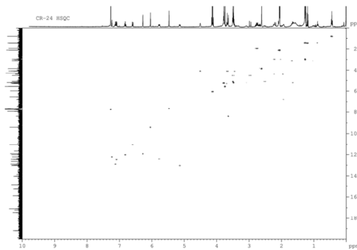
Figure 13. HSQC spectrum of 2
