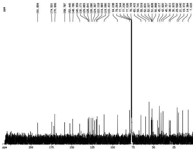
Figure 11. DEPT-135 spectrum of 2
