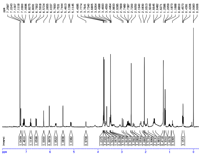
Figure 9. 1 H-NMR spectrum of 2
