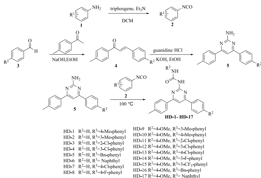
Scheme 1. Synthetic route of the target compounds
