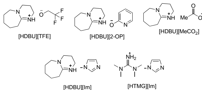
Figure 1. The protic ILs prepared in current study
