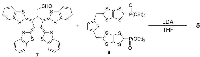
Scheme 1. Synthesis of 5
