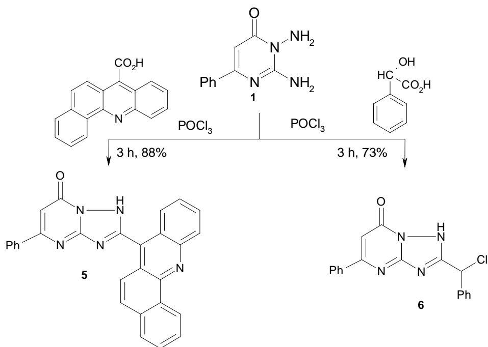
Scheme 2. Synthetic route for preparation of triazolopyrimidines 5 and 6
