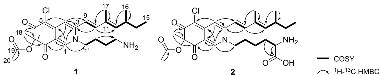
Figure 2. ^1\text{H} - ^1\text{H} COSY and key ^1\text{H} - ^{13}\text{C} HMBC correlations of 1 and 2
