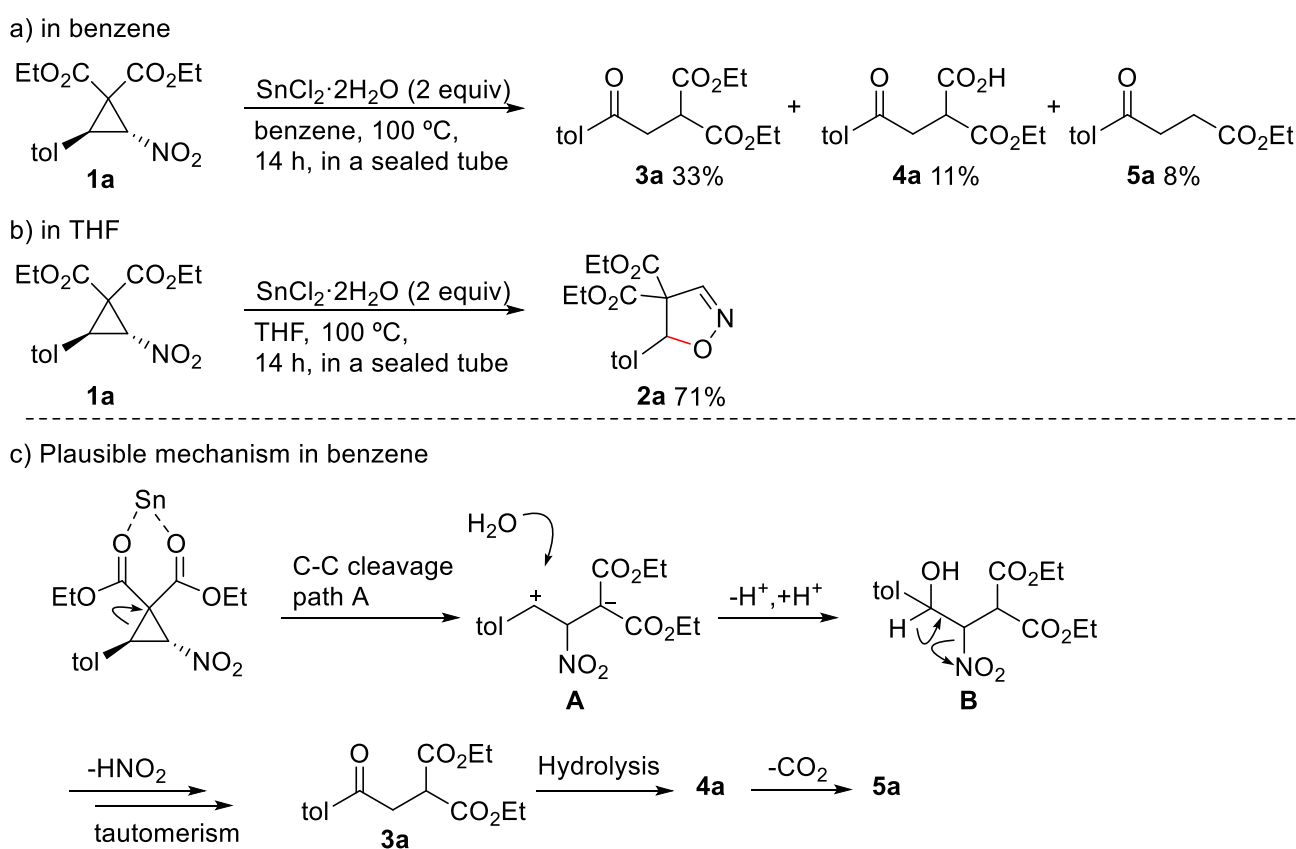
Scheme 2. Control experiments and plausible reaction mechanism for the formation of 3-5a
