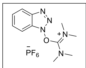
Figure 1. Structure of O -benzotriazole-1-yl)- N,N,N',N' -tetramethyluronium hexafluorophosphate (HBTU)
