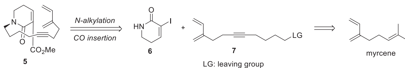
Scheme 3. Retrosynthetic analysis of compound 5 , the substrate of our proposed IMDA
