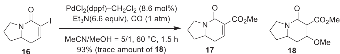
Scheme 6. Palladium-catalyzed carbonylation of 16 reported by Levinson et al. 9
