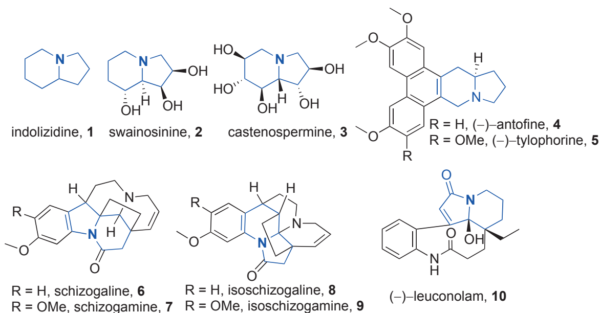
Figure 1. Indolizidine alkaloids
