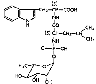
Phosphoramidon (1973)
