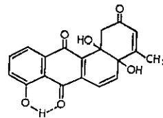
SS-228Y (1975)
