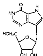
Formycin B (1966)
