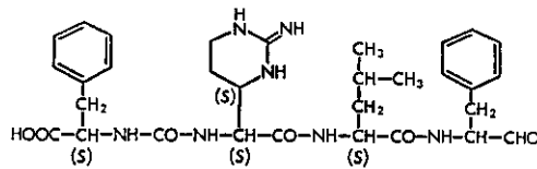
Chymostatin (1973)
