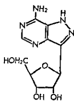
Formycin (1966)
