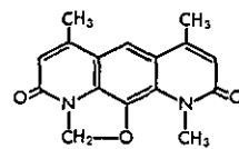
Deoxyrybomycin (1970)
