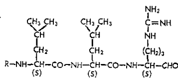
Leupeptins (1969)
