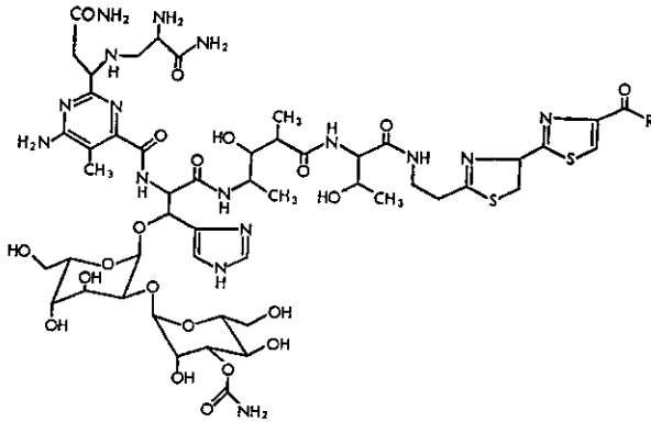
Phleomycins (1978)
