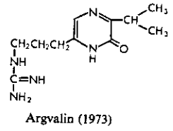
Argvalin (1973)
