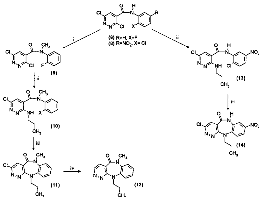
Scheme 3 i) KOH, DMSO, \text{CH}_3\text{I} , rt; ii) n\text{-C}_3\text{H}_7\text{NH}_2 , 1,4-dioxane, rt; iii) NaH, 1,4-dioxane, reflux; iv) \text{HCOONH}_4 , Pd-C, methanol, 48^\circ\text{C}
